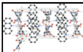
Fig. 4. A view along the b -axis of the crystal packing of the title compound. Hydrogen atoms not involved in the N—H...N and O—H...O hydrogen bonds (dashed lines) have been omitted for clarity (see Table 1 for details).
